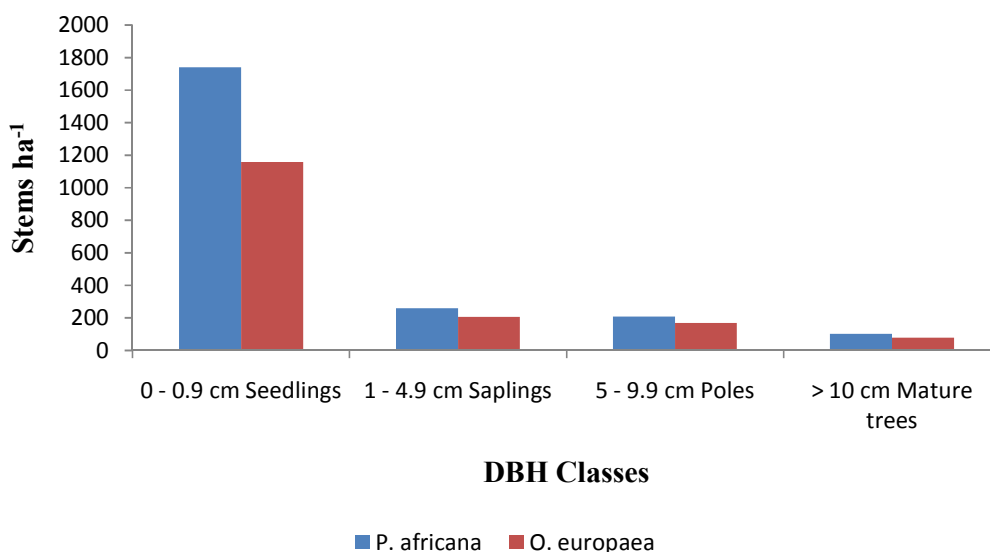
Fig. 5. Population density of P. africana and O. europaea in different size classes
