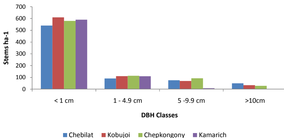
Fig. 4. Population density of Olea europaea in each DBH class in four sites
