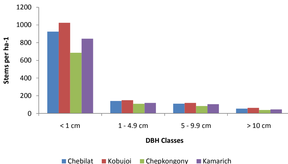
Fig. 3. Population density of Prunus africana in each DBH class in four sites
