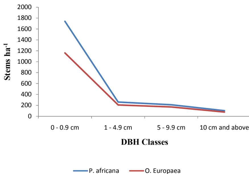
Fig. 6. Diameter size class distribution profile for Prunus africana and Olea europaea
