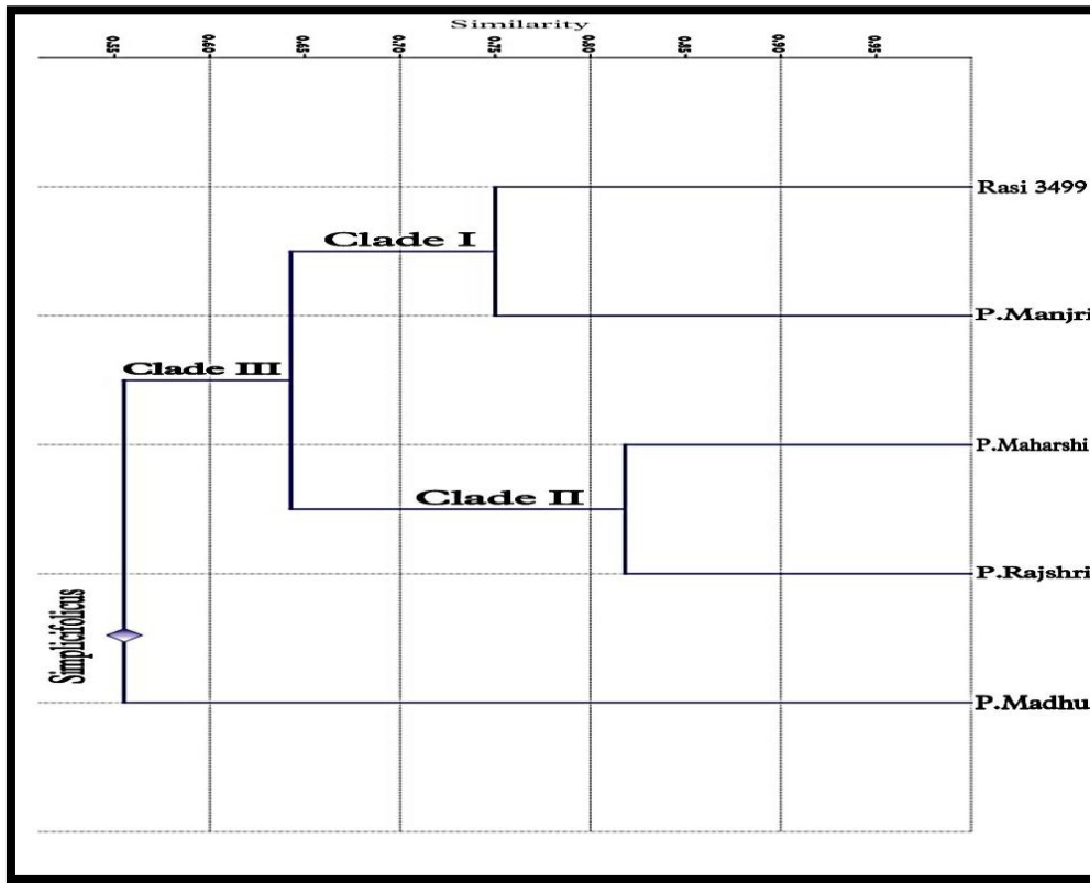
Fig. 2. Dendrogram generated using UPGMA analysis showing relationship among maize varieties using SSR marker
