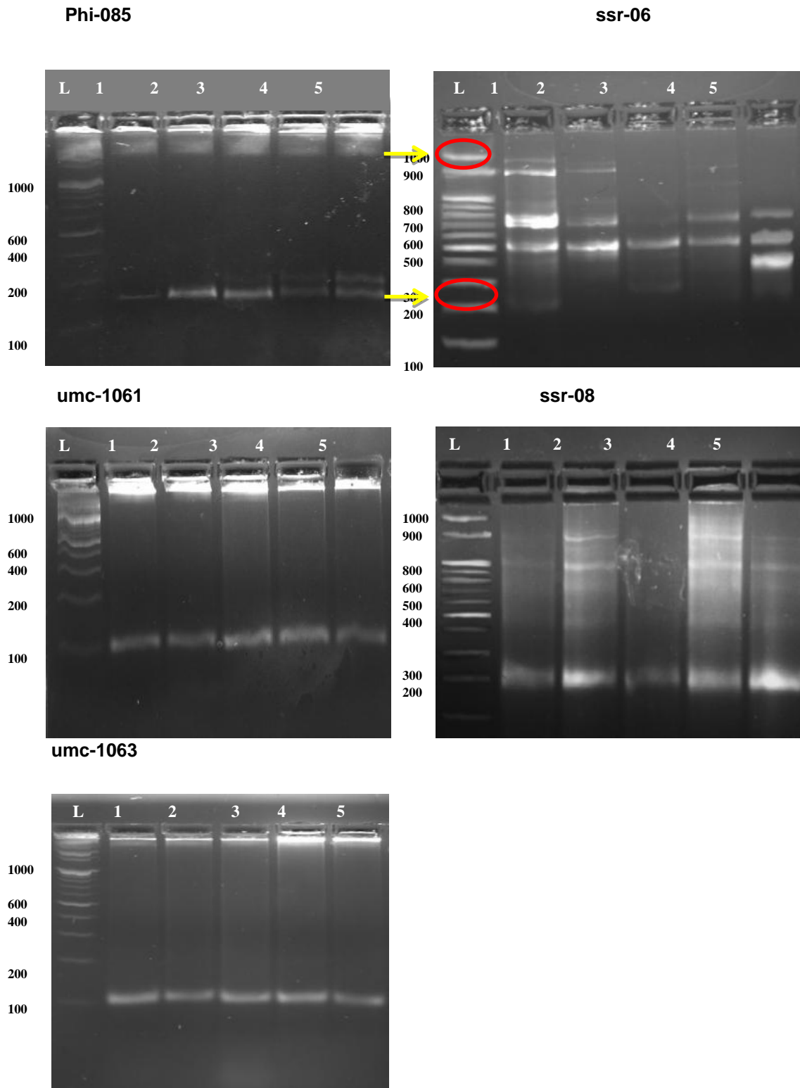
Fig. 1. PCR amplification of maize varieties using SSR markers (L-100 bp ladder, 1-P. Rajshri, 2-P.Madhu, 3-P.Maharshi, 4-P.Manjri, 5- Rasi-3499)
