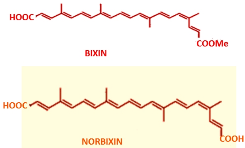
Fig. 2. Chemical structure of Bixin and Norbixin.
