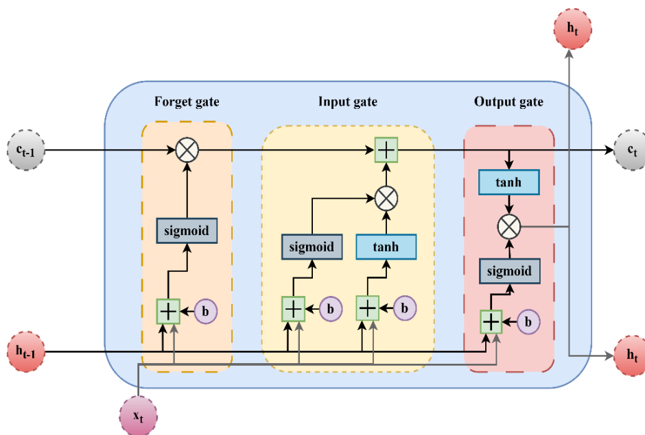
Fig. 3. LSTM architecture
