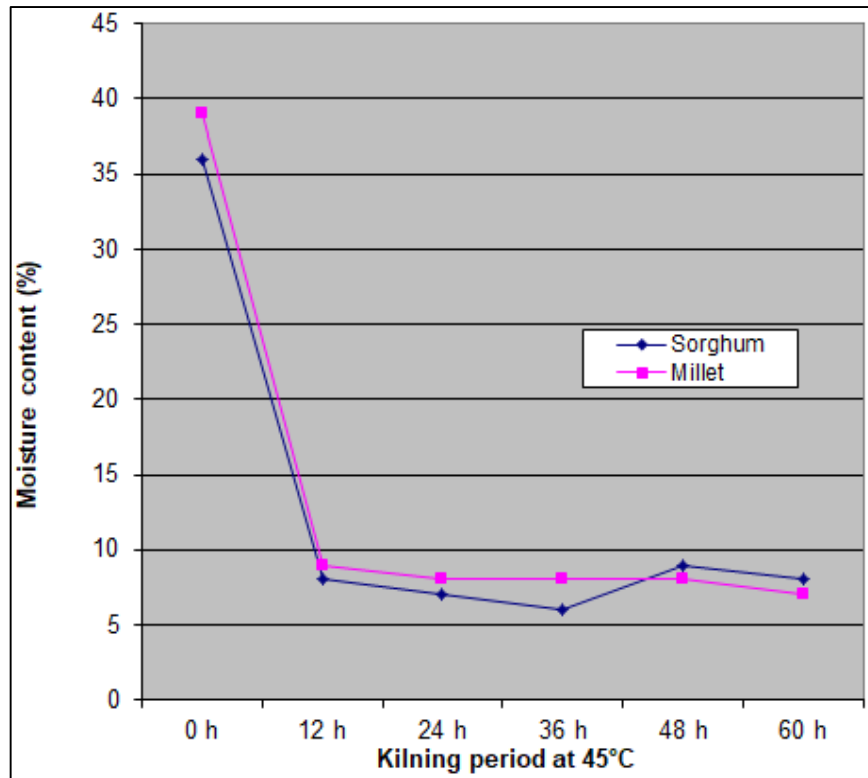
Fig. 5. Moisture content (%) against kilning periods (h) at 45°C
