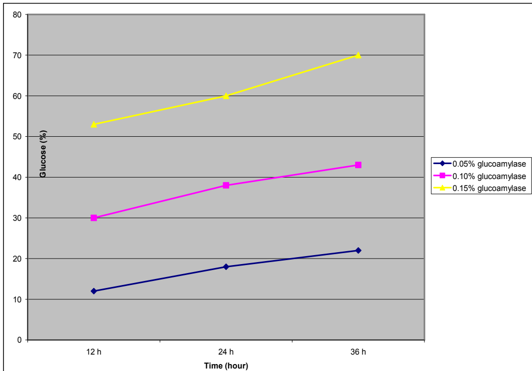
Fig. 9. Effect of varying concentrations of glucoamylase and saccharification time on the reducing sugar content of the syrup
