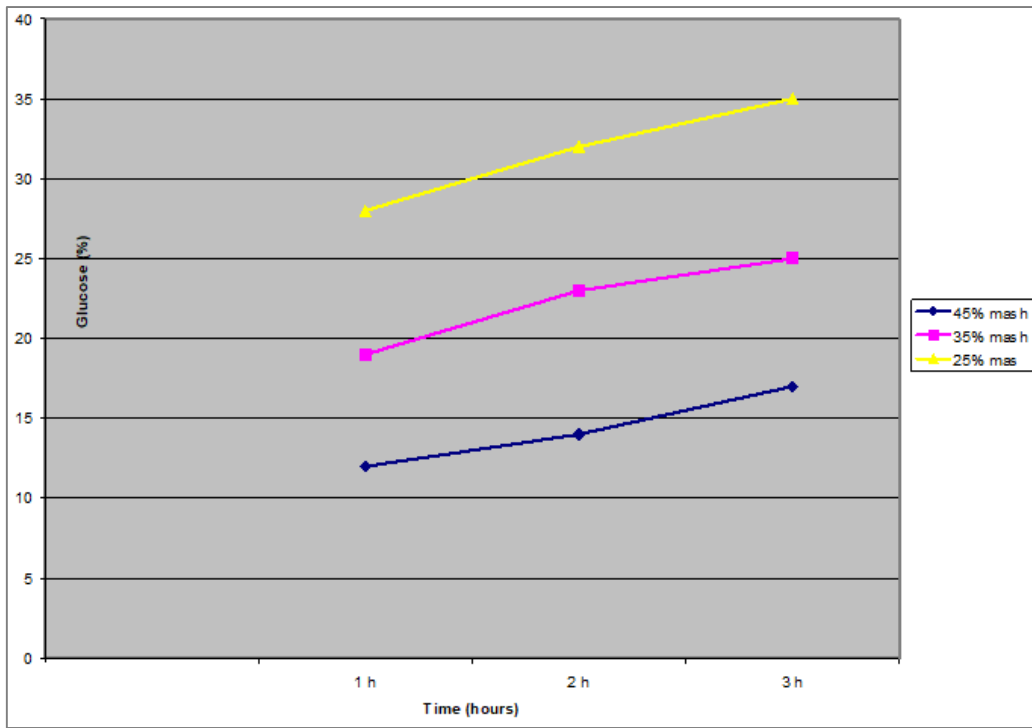
Fig. 8. Effect of varying mash concentrations and saccharification time on reducing the sugar content of the wort
