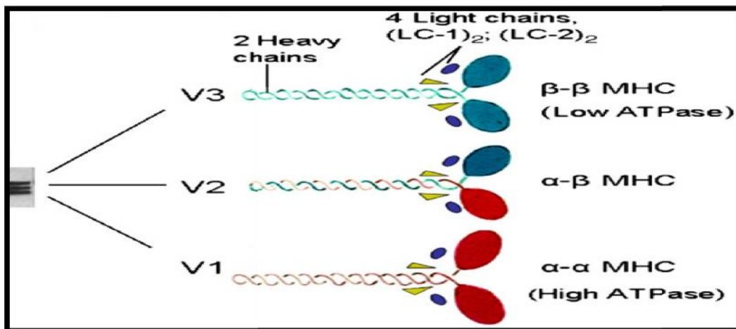
Fig. 1. MHC structure [9]
