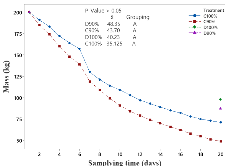
Fig. 6. Mass reduction of different manure and wood shavings mixing ratios during composting and dumping. D100: dumped raw manure, D90: 90% raw manure dumped with 10% wood shavings, C100: composted raw manure, C90: 90% raw manure composted with 10% wood shavings
