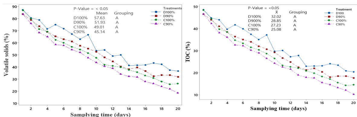
Fig. 8. Volatile solids (VS) and Total organic carbon (TOC) variation of different manure and wood shavings mixing ratios during composting and dumping. D100: dumped raw manure, D90: 90% raw manure dumped with 10% wood shavings, C100: composted raw manure, C90: 90% raw manure composted with 10% wood shavings
