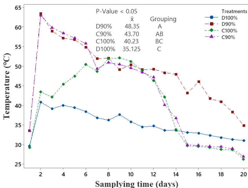
Fig. 3. Variation in pile manure temperature of different manure and wood shavings mixing ratios during composting and dumping. D100: dumped raw manure, D90: 90% raw manure dumped with 10% wood shavings, C100: composted raw manure, C90: 90% raw manure composted with 10% wood shavings
