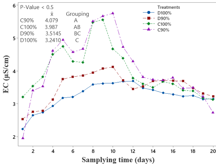
Fig. 5. Variation in Electrical conductivity of different manure and wood shavings mixing ratios during composting and dumping. D100: dumped raw manure, D90: 90% raw manure dumped with 10% wood shavings, C100: composted raw manure, C90: 90% raw manure composted with 10% wood shavings
