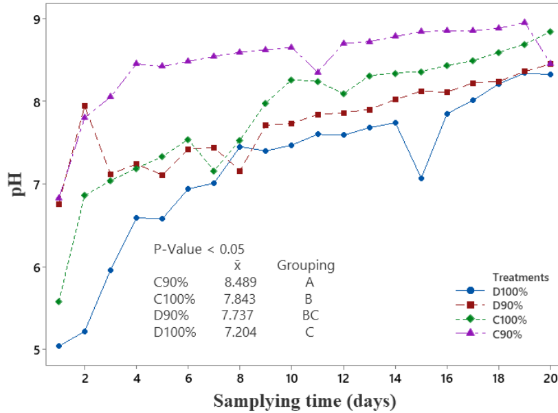
Fig. 4. Variation in pH of different manure and wood shavings mixing ratios during composting and dumping. D100: dumped raw manure, D90: 90% raw manure dumped with 10% wood shavings, C100: composted raw manure, C90: 90% raw manure composted with 10% wood shavings
