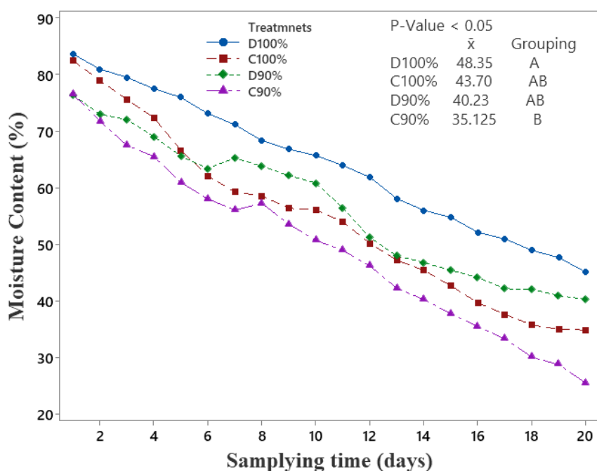
Fig. 7. Moisture content variation of different manure and wood shavings mixing ratios during composting and dumping. D100: dumped raw manure, D90: 90% raw manure dumped with 10% wood shavings, C100: composted raw manure, C90: 90% raw manure composted with 10% wood shavings
