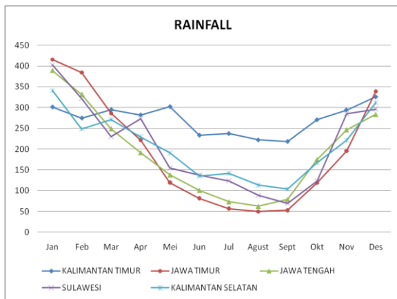
Figs. 1, 2. Graph average Rainfall and Temperature on 5 Provinces Rice Production in Indonesia [4]
