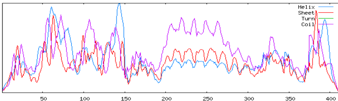
Fig. 2. Secondary structure of vaccine construct using SOPMA server
