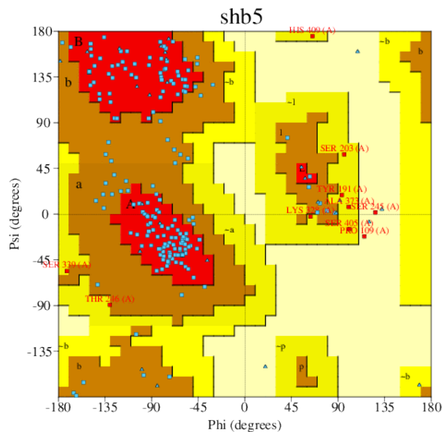
Fig. 4. Ramchandran plot of refined model using PDBSum
