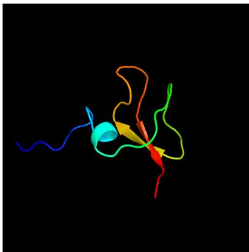
Fig. 3. Tertiary structure of vaccine construct using Phyre2 server
