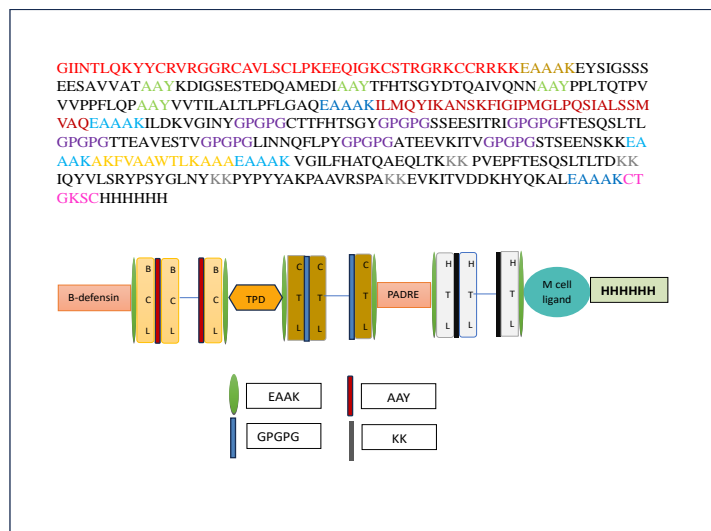
Fig. 1. Multiprotein multi-epitope vaccine construct. With color coding for different adjuvants and epitopes
