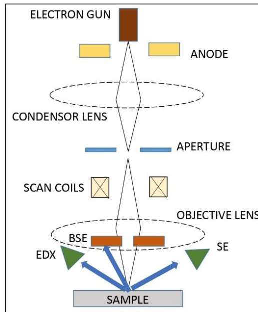
Fig. 1. Schematic diagram of SEM-EDX. A beam of electrons is produced at the top of the microscope by an electron gun mounted in an enclosure and maintained at high vacuum. The beam travels through electromagnetic fields and lenses, which focus the beam towards the sample. All electromagnetic lens and detector are maintained at high vacuum. There are three main signals that occur when an electron beam meets the sample
