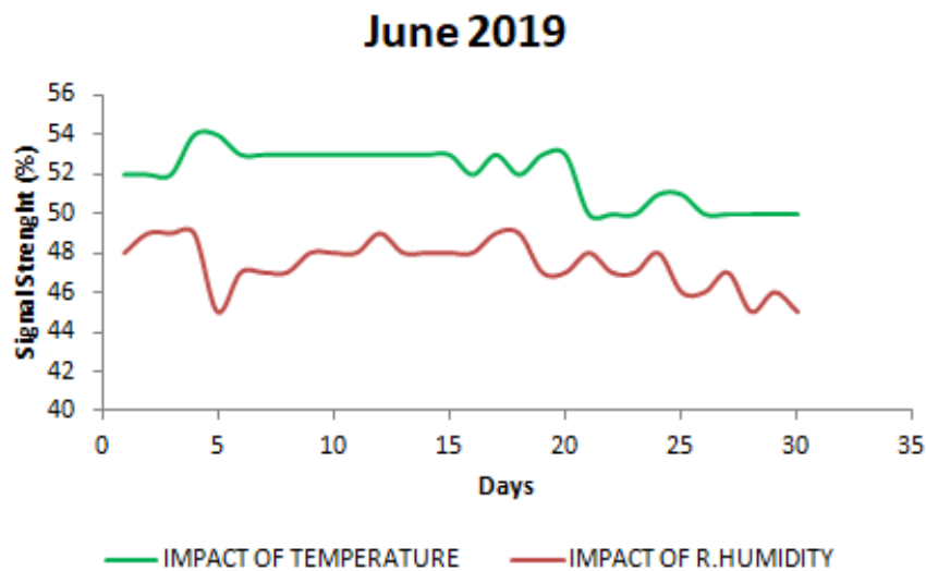
Fig. 3. Comparing the effects of temperature and relative humidity on RSS for June, 2019
