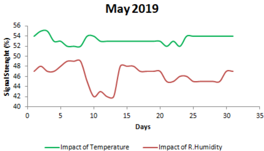
Fig. 2. Comparing the effects of Temperature and Relative humidity on RSS for May, 2019
