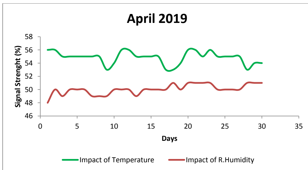
Fig. 1. Comparing the effects of temperature and relative humidity on RSS for April, 2019
