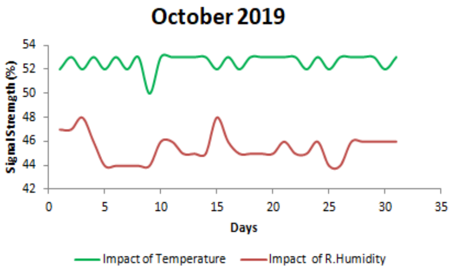
Fig. 4. Comparing the effects of temperature and relative humidity on RSS for October 2019
