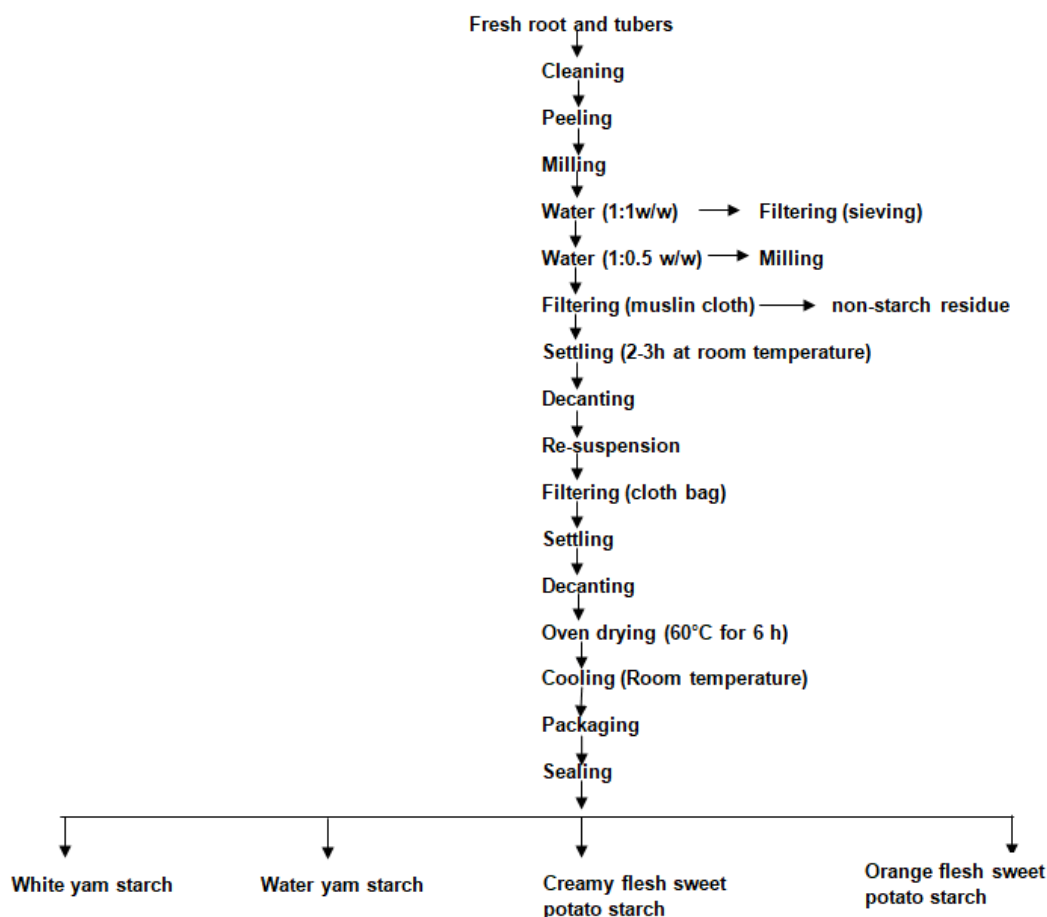
Fig. 1. Flow process of starch production for root and tubers
