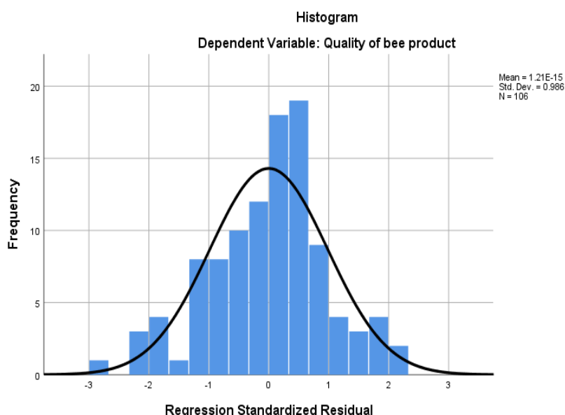
Fig. 2. Normality test
