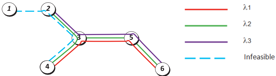
Fig. 1. Unroutable 1-4 traffic due to wavelength-continuity constraints [2,8]
